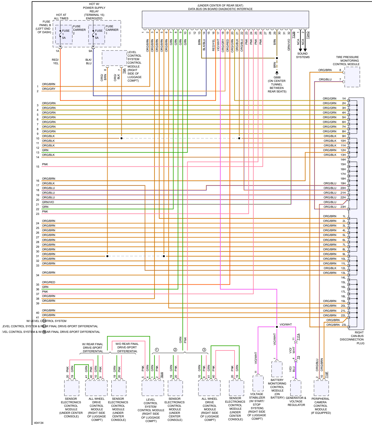
Fig 4: Computer Data Lines Circuit (4 of 4)
